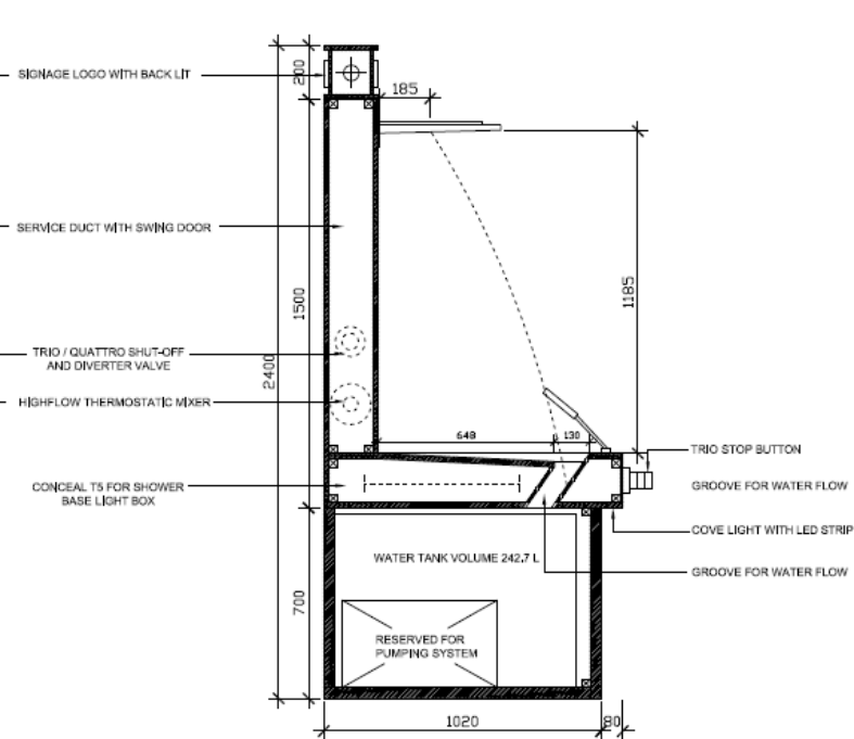
SECTION X-X
