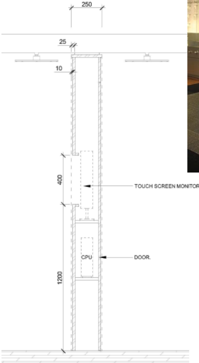
SECTIONAL VIEW
