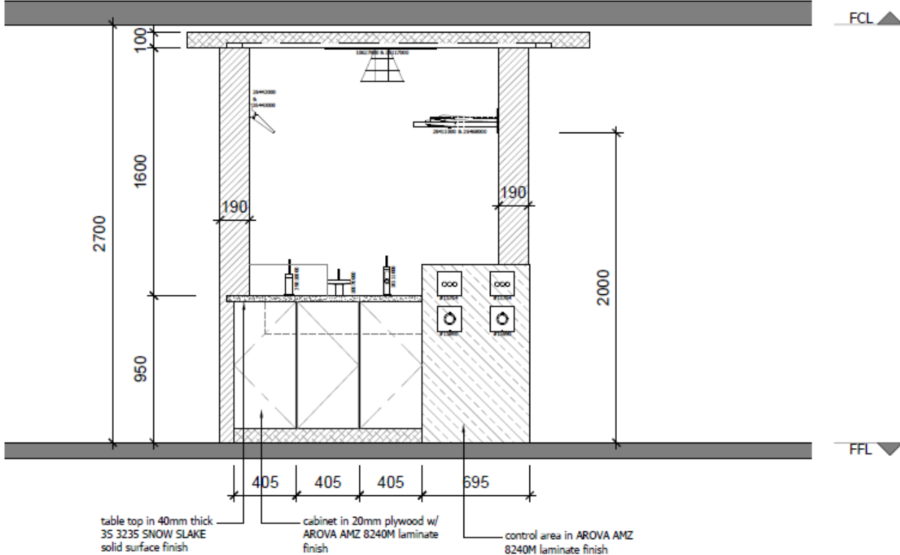
LIVE DEMO ELEVATION A (AS BUILT) SCALE: 1:20
