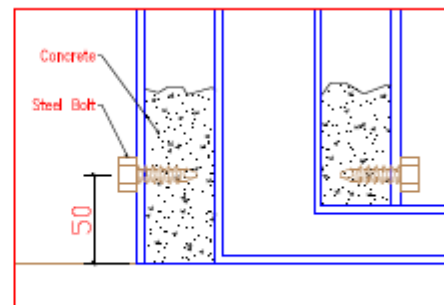
Detail 02
