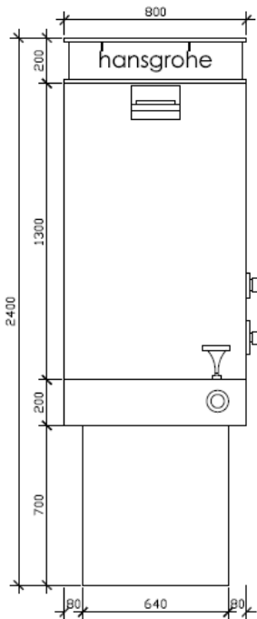
FRONT ELEVATION
