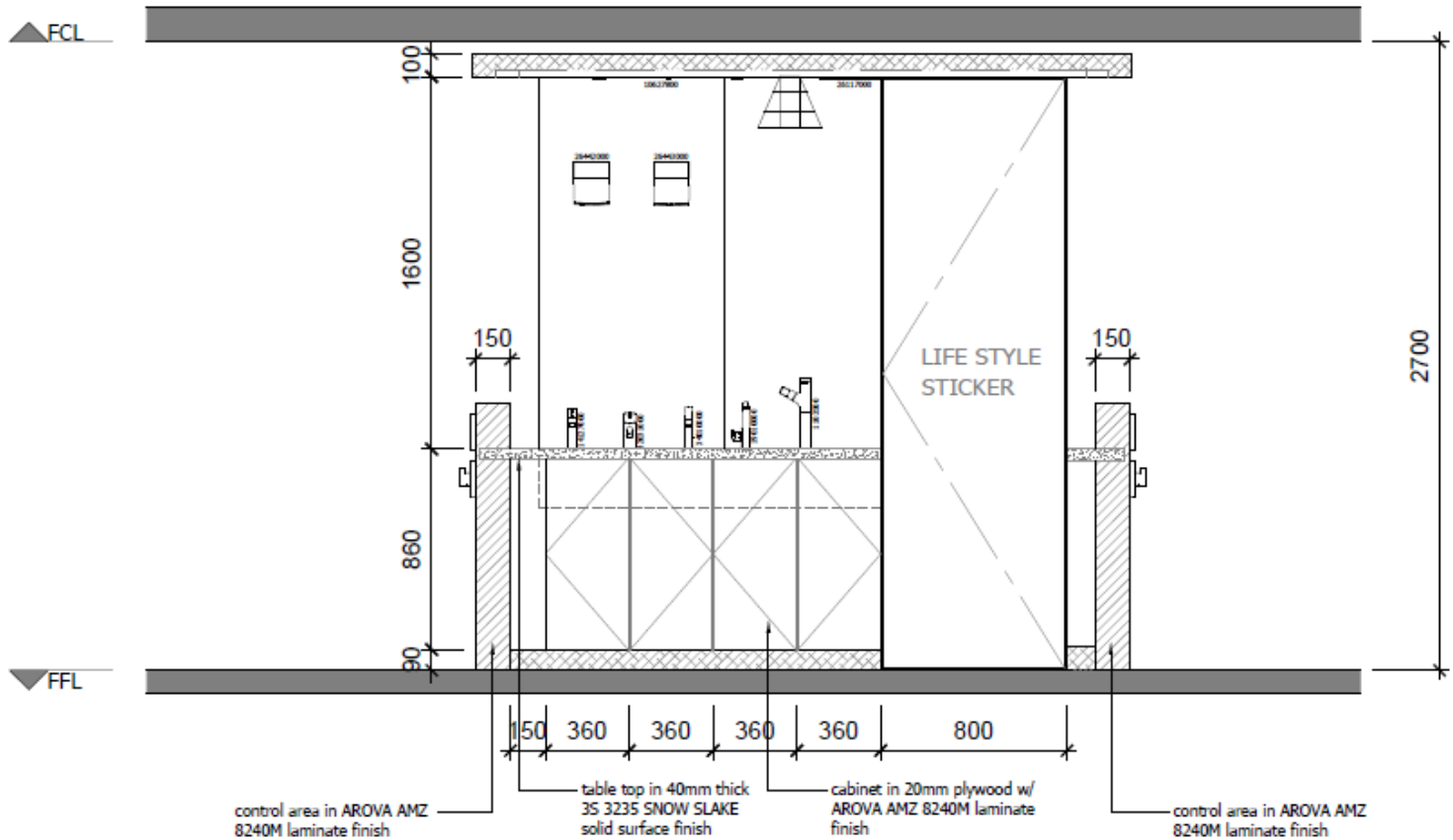
LIVE DEMO ELEVATION D (AS BUILT) SCALE: 1:20
