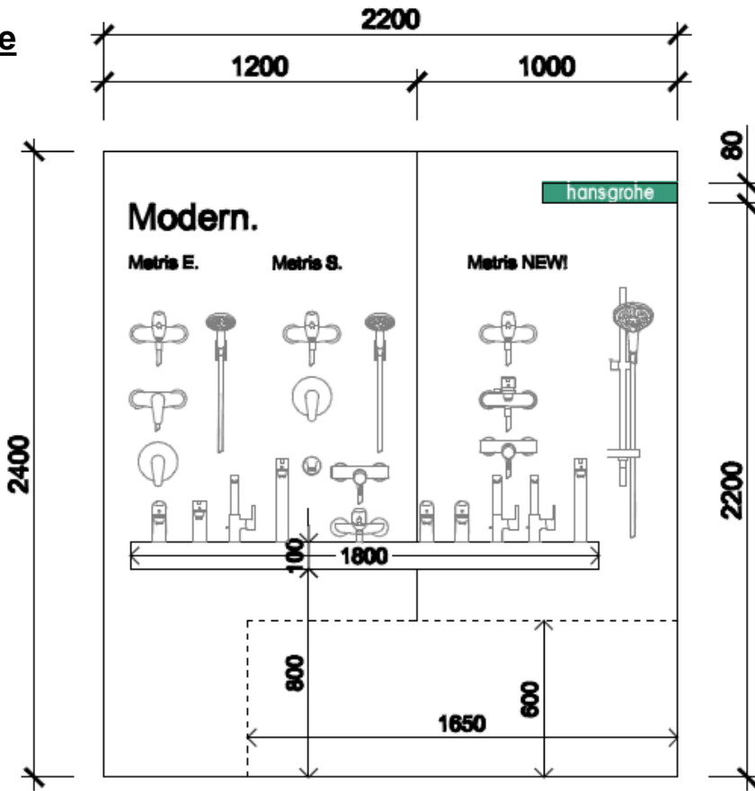
FRONT ELEVATION
