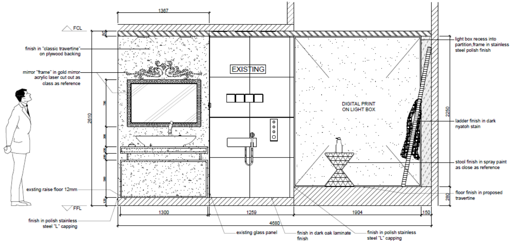
EXHIBITION ELEVATION A SCALE: 1:20
