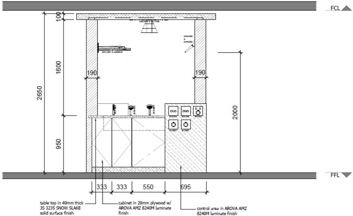
LIVE DEMO ELEVATION C(AS BUILT) SCALE: 1:20
