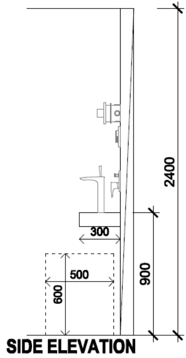
SIDE ELEVATION
